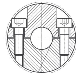
Splitnav
